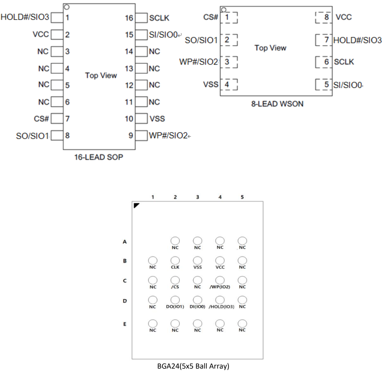
Figure 6.1 Pin Configuration
